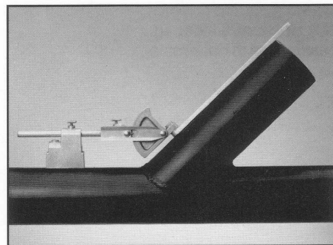
FITTER WELDER PROTRACTOR 0721-0008 . . . . . Stock No. 9
